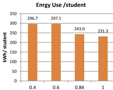
Figure (7) Total annual energy use, at WWR 25%, and different occupancy densities for East orientation
