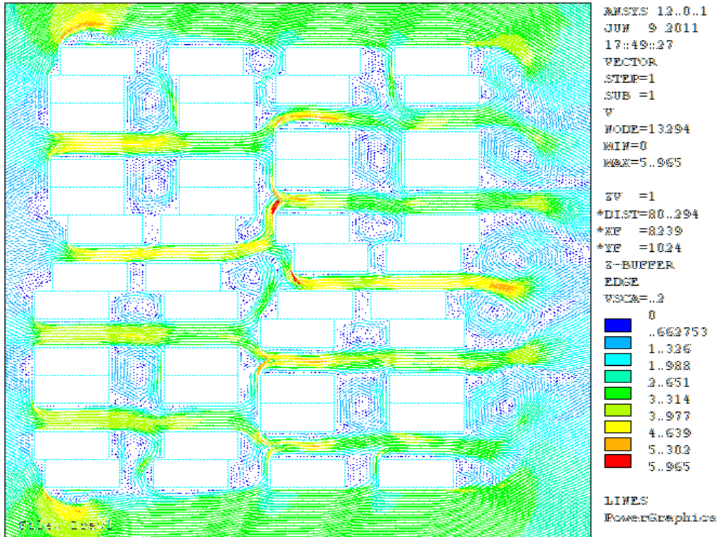
Fig.4. the vectors of Air flow pattern through row houses urban pattern.
